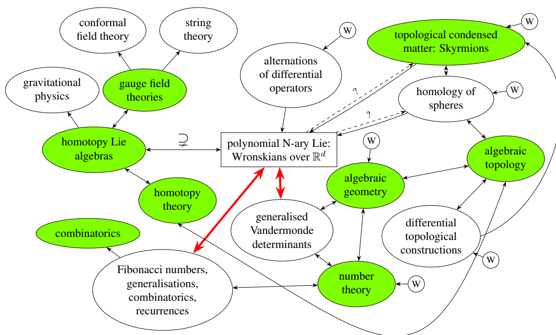
FIGURE 1. Relation of polynomial N -ary Lie algebras – with generalised Wronskian brackets – as higher structures in physics to other fields of physics and mathematics (shaded in green ) and specific theories and constructions within them (not shaded). The symbol ‘W’ denotes that Wronskian determinants naturally appear in the field (cf. [6]); arrows highlighted in thick red indicate that (to the best of our present knowledge) we were the first to find the connection.
